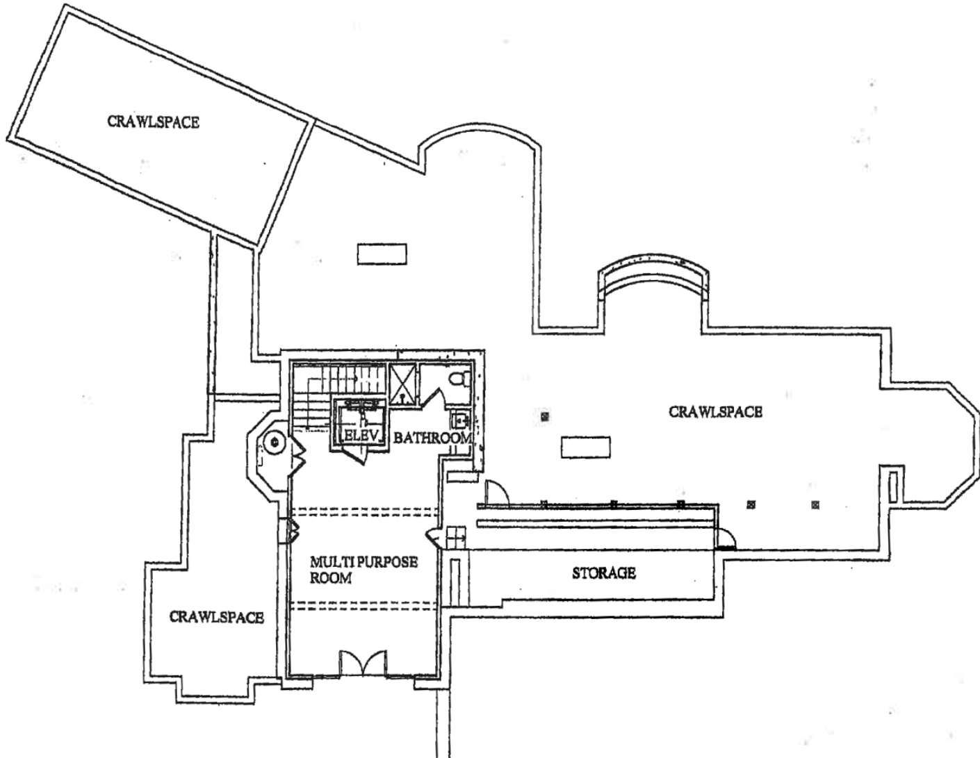
1 MAIN HOUSE BASEMENT FLOOR PLAN 3/32" = 1'-0"
